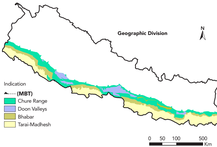
FIGURE 3.3. GEOLOGICAL AND GEOGRAPHIC DIVISION OF CHURE RANGE AND CB REGION
